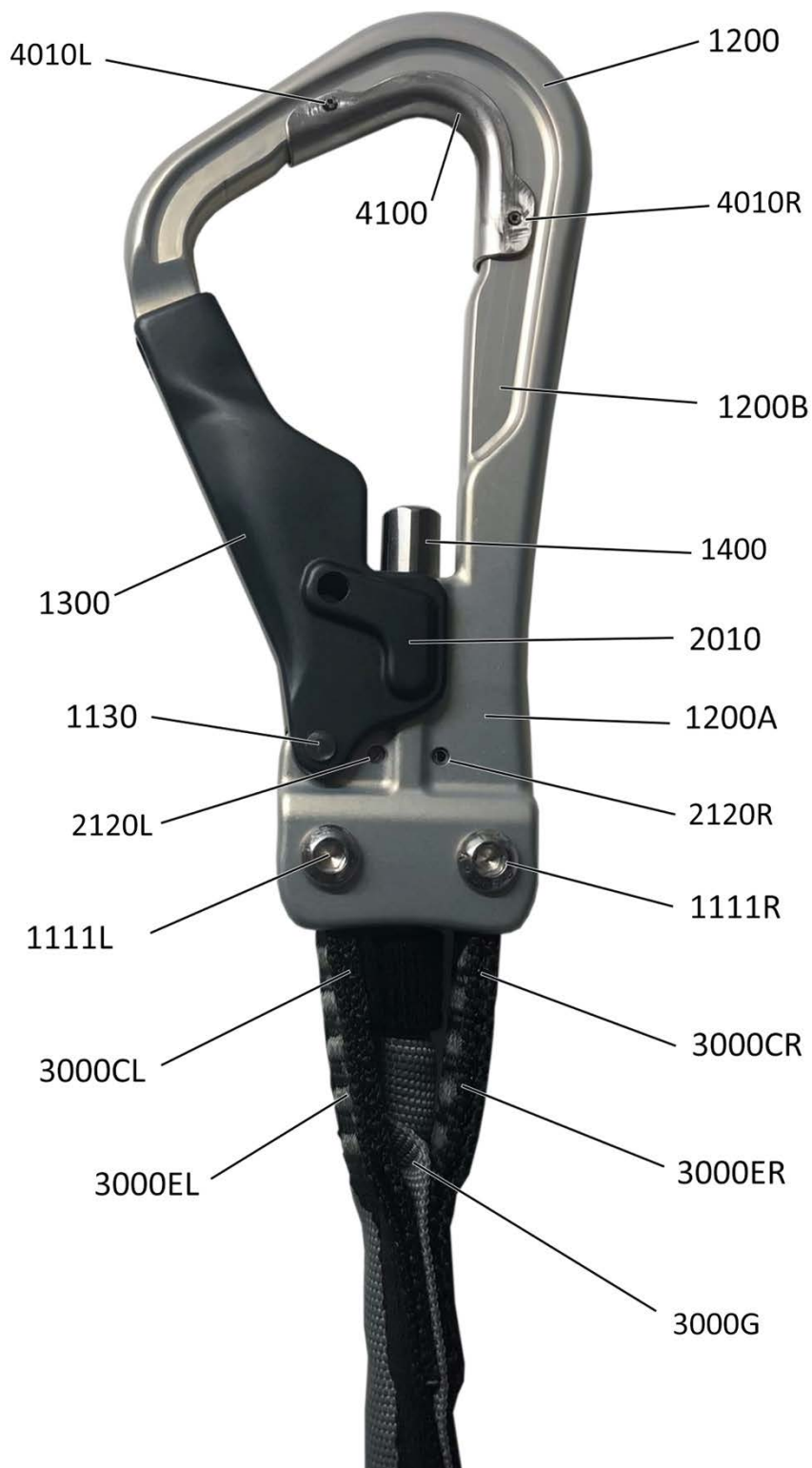
Figure 4: Carabiner Head
