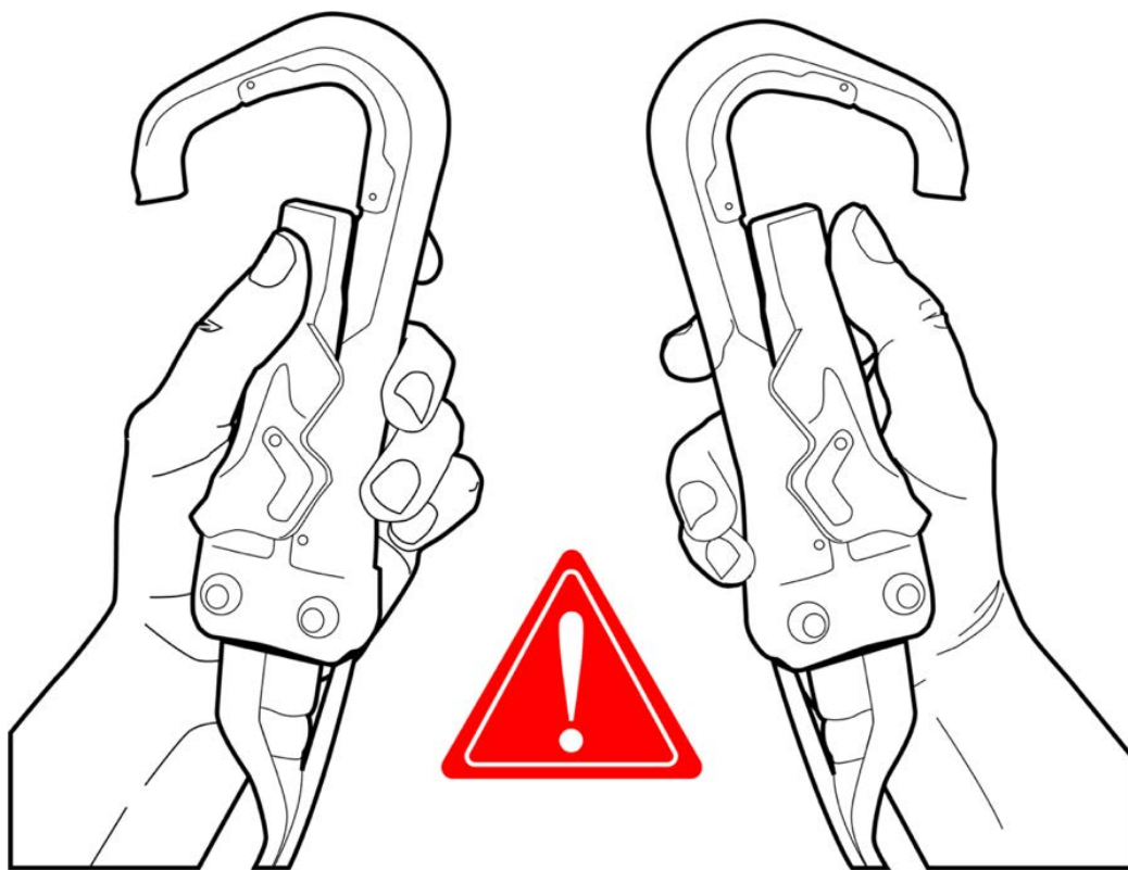
Figure 25: Alpha error
